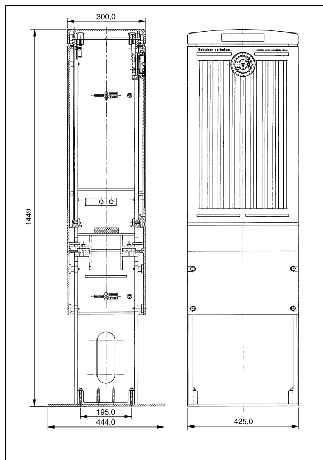
Cabinet 92AR with cable head rack, door version with half profile cylinder
