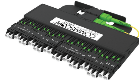
Figure 13: Right-exit MPO module with LC adaptors
