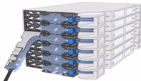
Figure:17: Installed FACT-FRACCCTU6E with cable exit in the left bottom corner.
