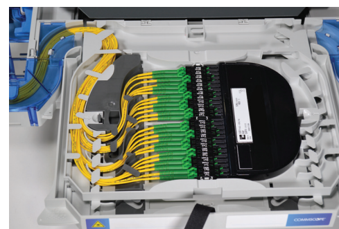
Figure 14: Value-added module shown loaded into a FACT NG4 chassis
