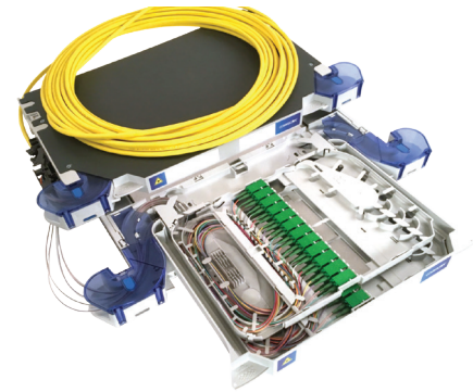
Figure 9: Two-element pre-cabled chassis with 96 indoor microsheet cable and right-side patching
